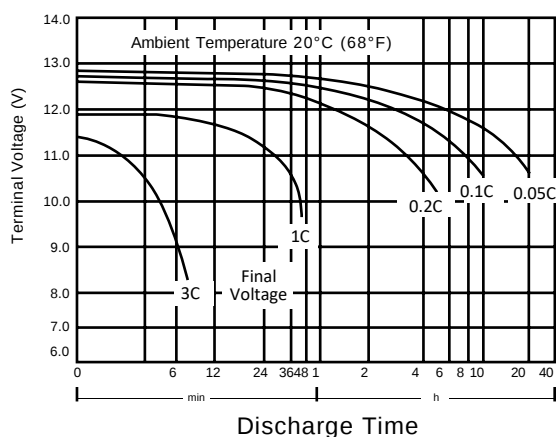
Discharge Characteristics
